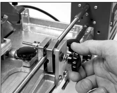
Fig. 10. Loosen clutch plate
