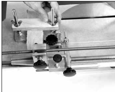
Fig. 16. Material positioned in vise near blade prior to cutting
